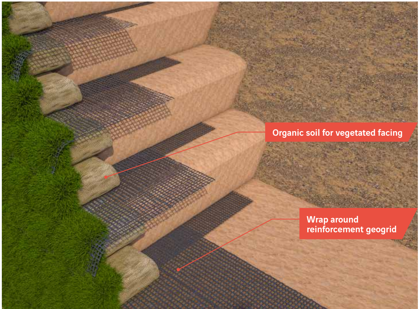
ArmaGreen with wrapped geogrid reinforcement.
